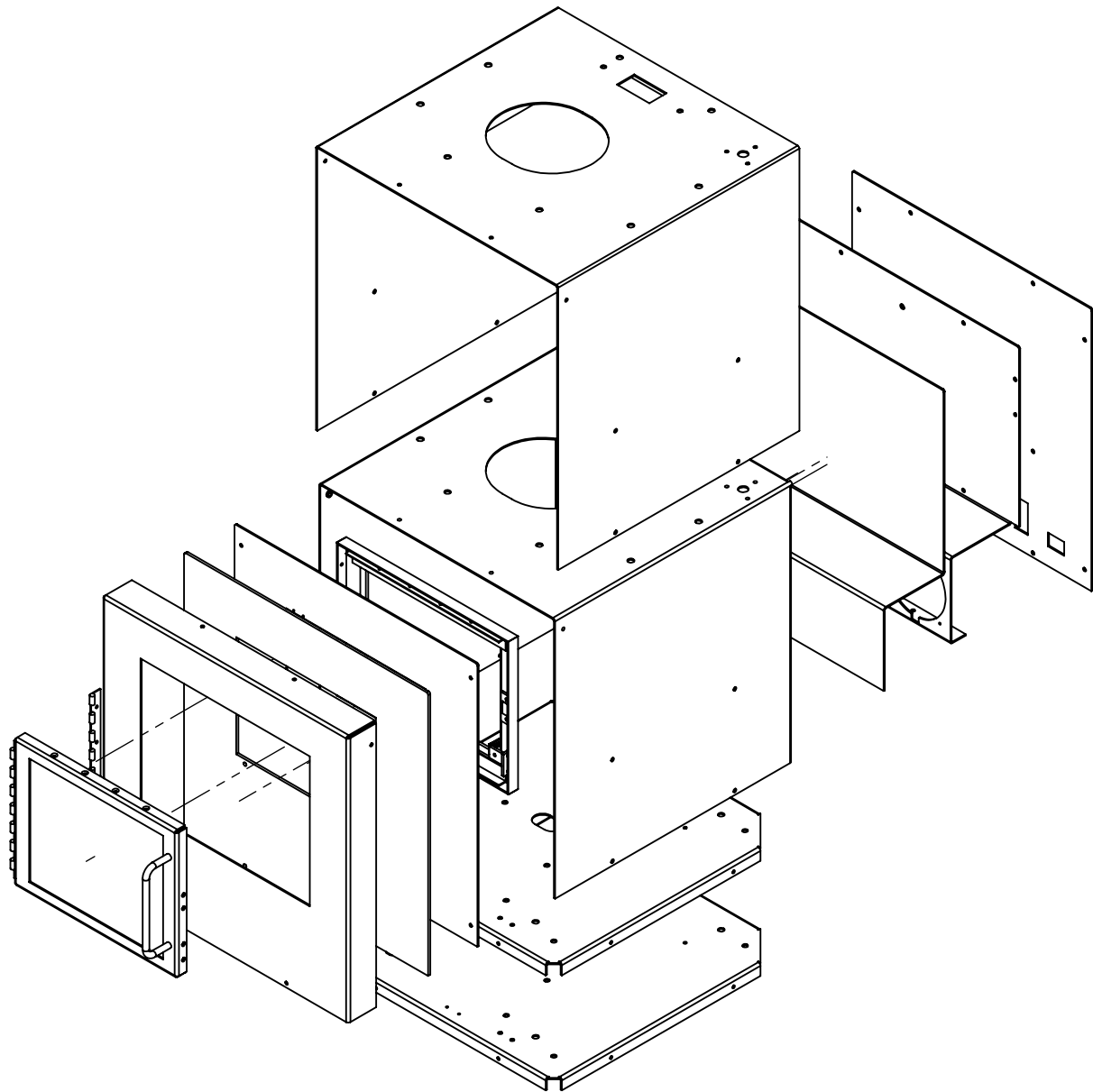
SHEET METAL
